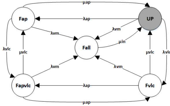
Figure 3: CTMC model for the Service module.
